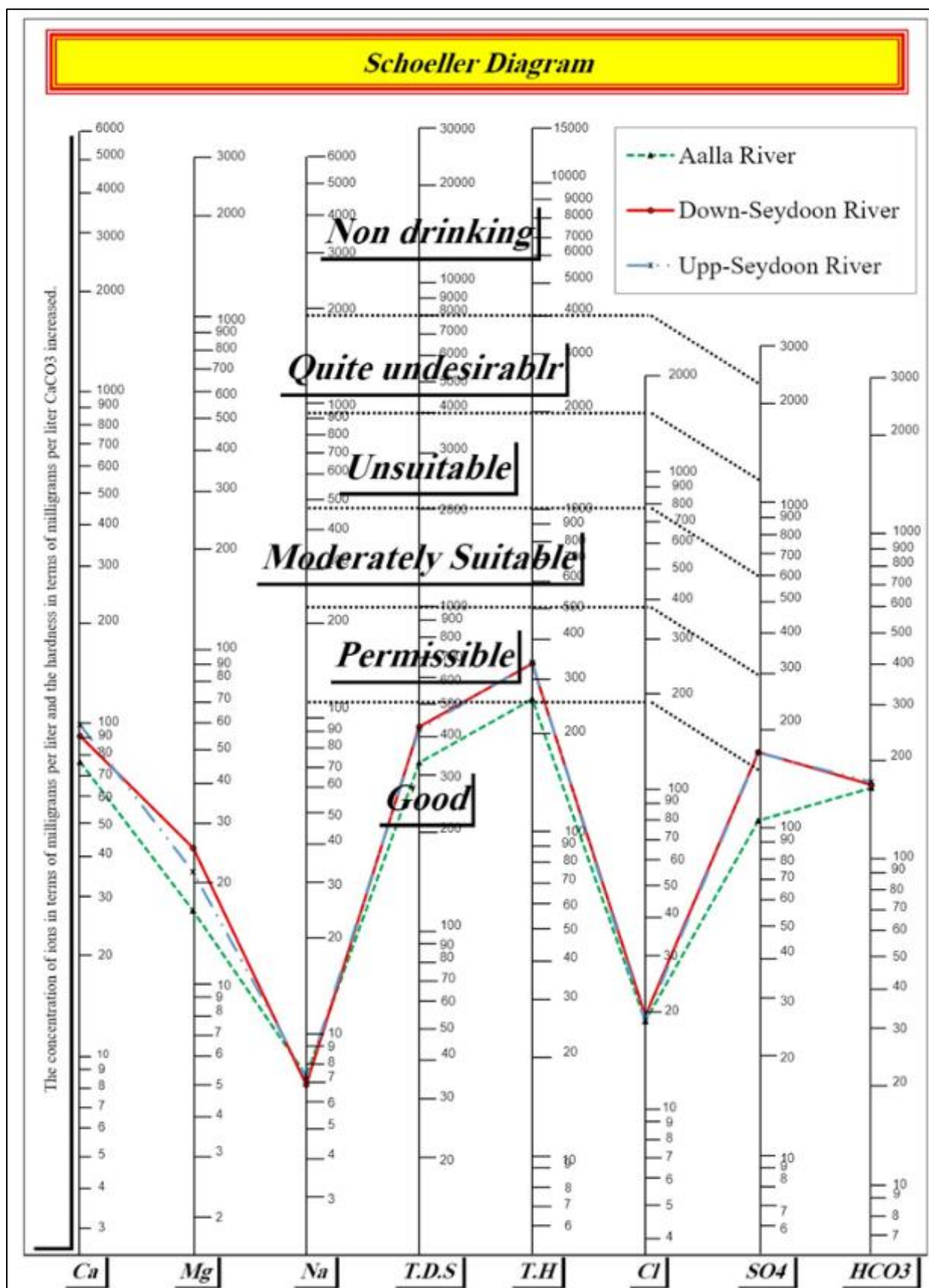
Figure 3 Schuler diagram of water samples from the Seydoon River and the Alaa River
