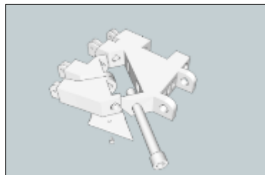
Figure 3 CAD design for the palm shows the hinge for the 4th and 5th fingers, showing how the palm is put together
