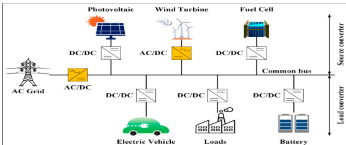
Figure 1 Schematic diagram of DC microgrid
