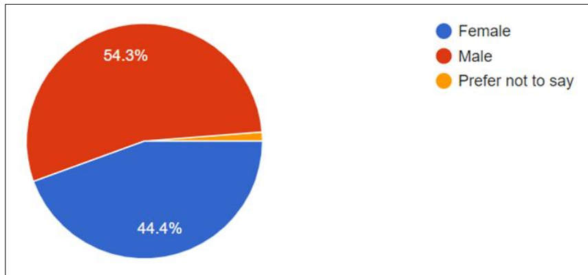
Figure 2 44 male and 36 female participants completed the questionnaire
